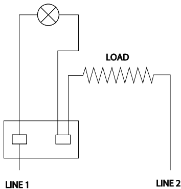
PILOT LIGHT (OPTIONAL) IS ON WHEN THERMOSTAT SWITCH IS OFF
